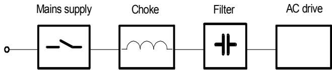
Figura 6.2: Inverter
