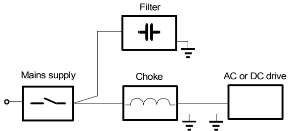
Figure 6.3: ECF filter
